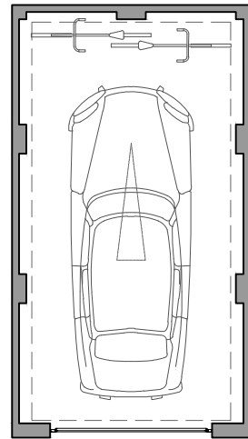
Single Garage *Garages also provide x2 cycle spaces Floor Plan
